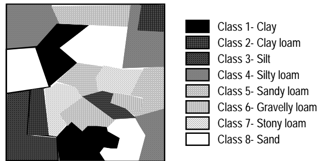
Figure 1. Simple soils map.
