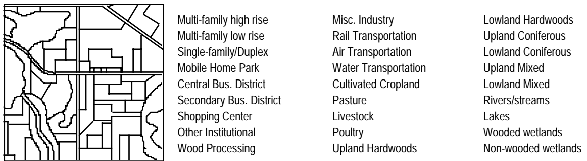
Figure 2. Land use/land cover map and list of categories (adapted from Anderson(1976)).
