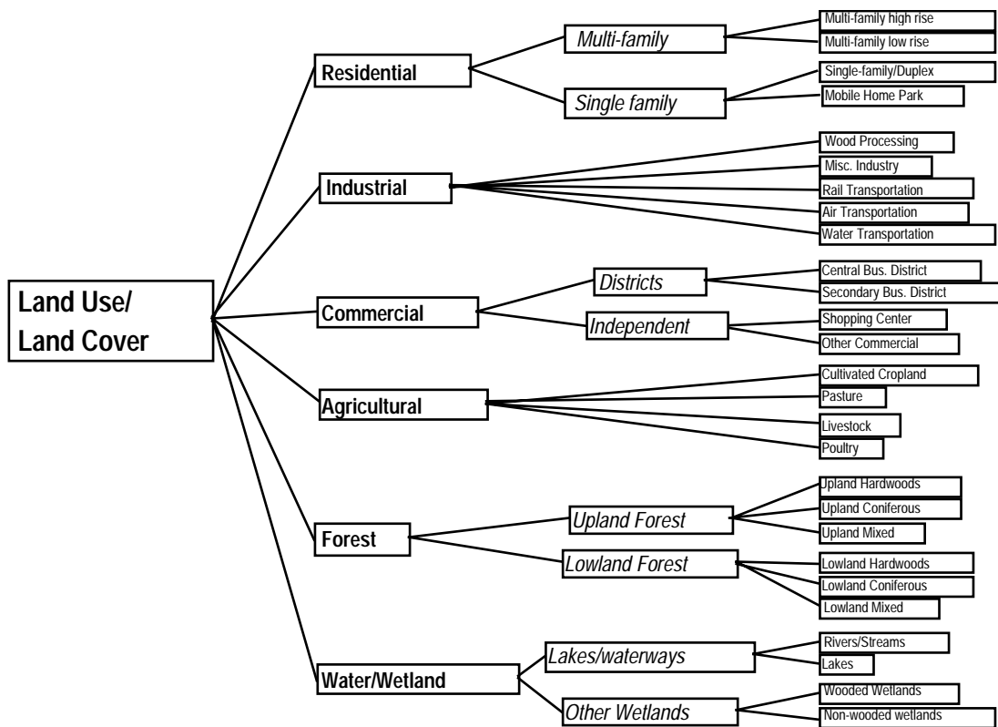
Figure 13. Hierarchical attribute domain taken from Figure 6.
