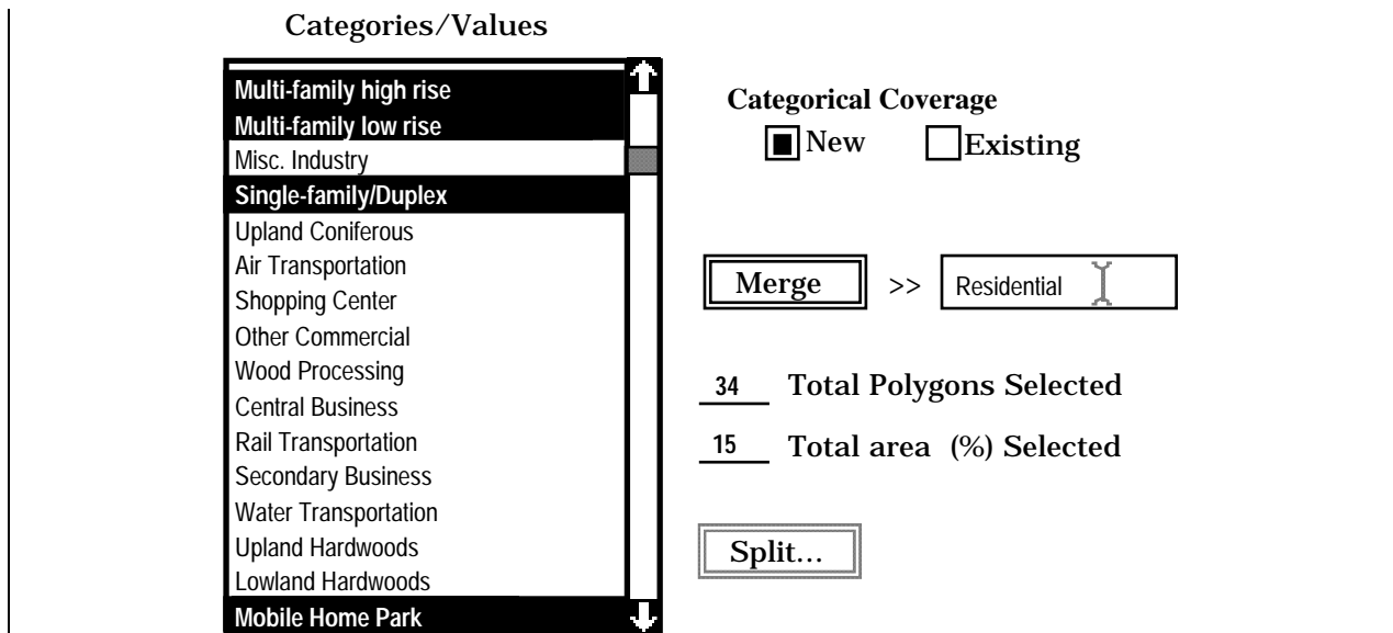
Figure 12. One possible implementation for category manipulation
